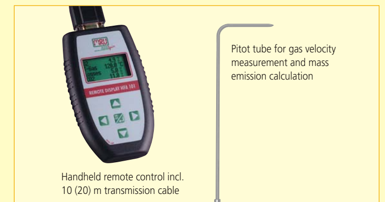
Differential pressure measurement for Pitot tube connection
